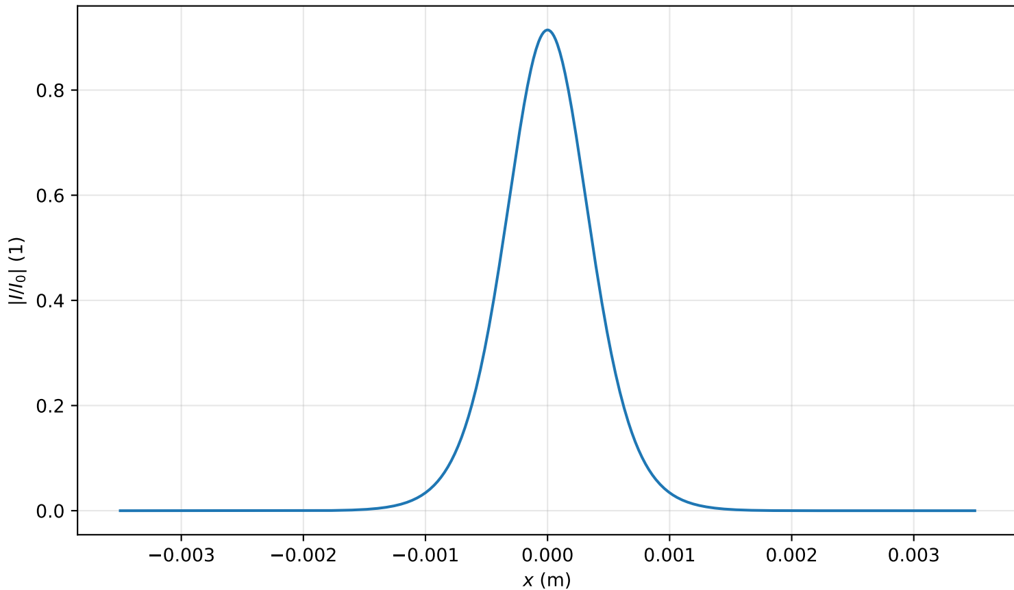
Intensity profile I(x, y = 0, z = 1.672m)/I_0 , P_{in}=0.5P_{cr} , artificial time
